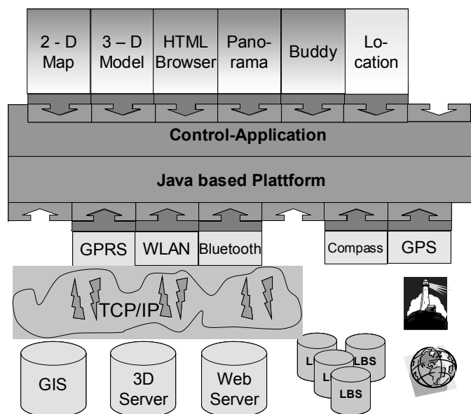
Figure 1. The Niccimon mobile test platform architecture
